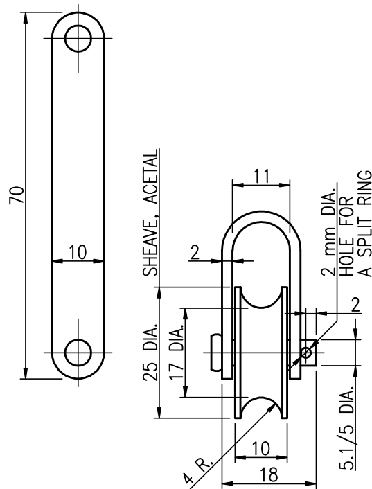
JIB HALLIARD AND KICKING STRAP BLOCKS STAINLESS STEEL
