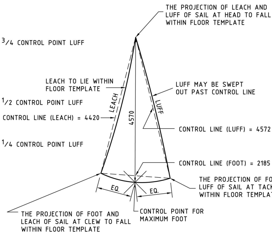
HEADSAIL
