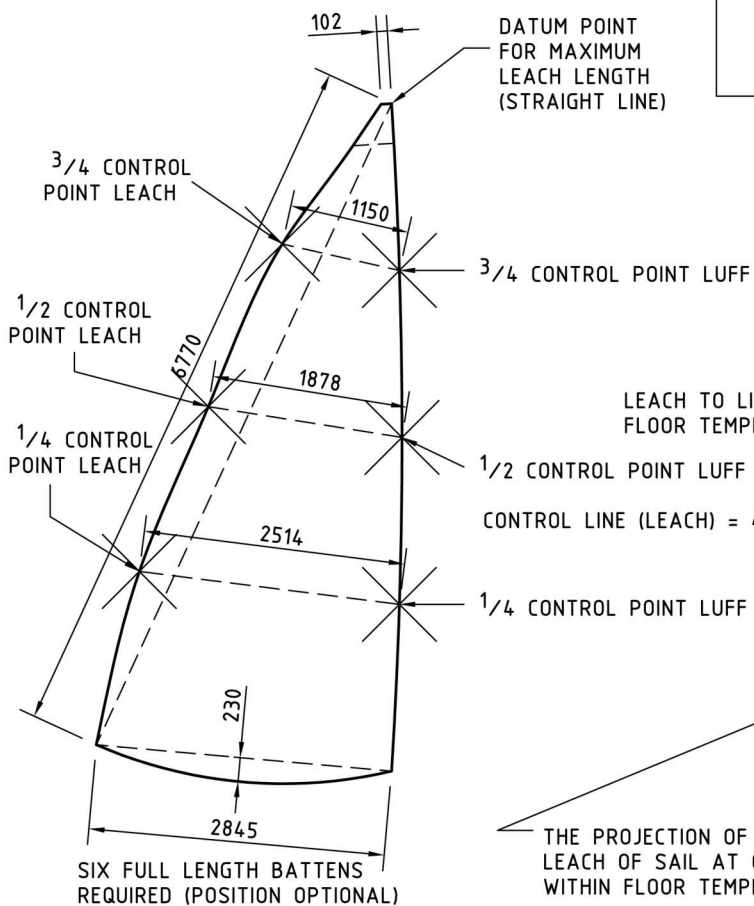
MAINSAIL
