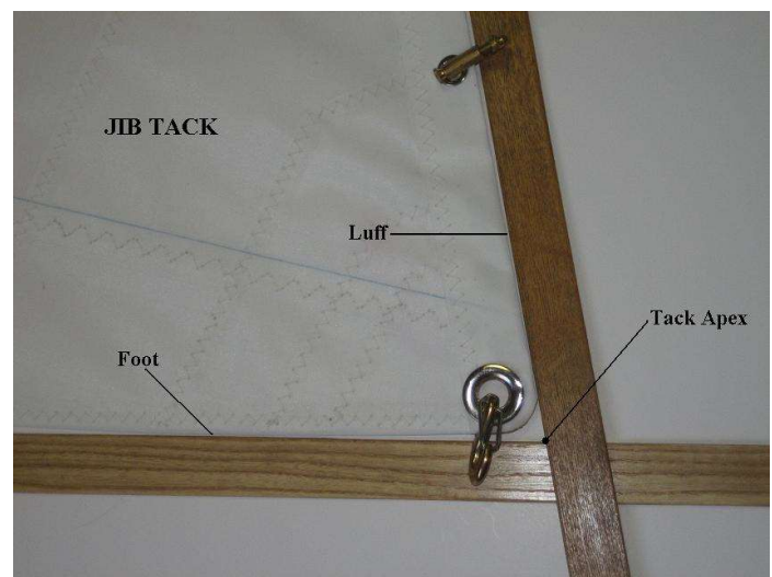
Figure 4c – Jib Tack
