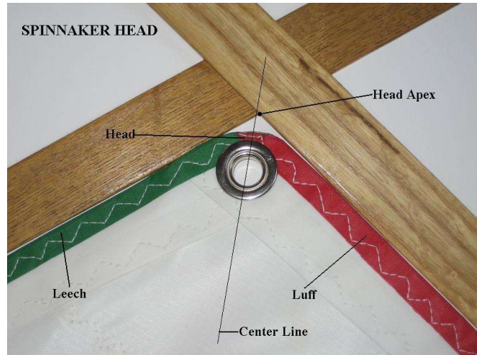
Photo 7 – Spinnaker Head
