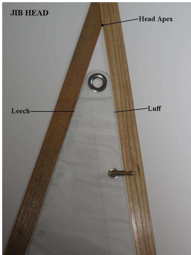
Figure 4a – Jib Head
