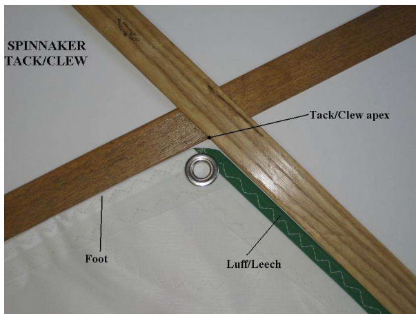
Photo 8 - Spinnaker Clew
