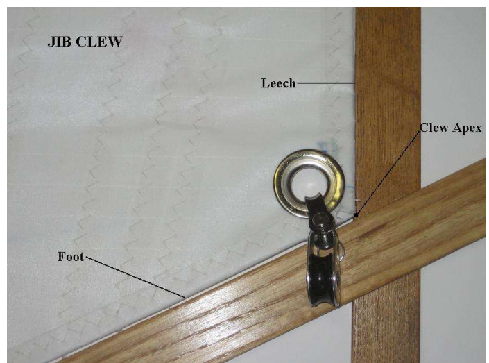
Figure 4b – Jib Clew
