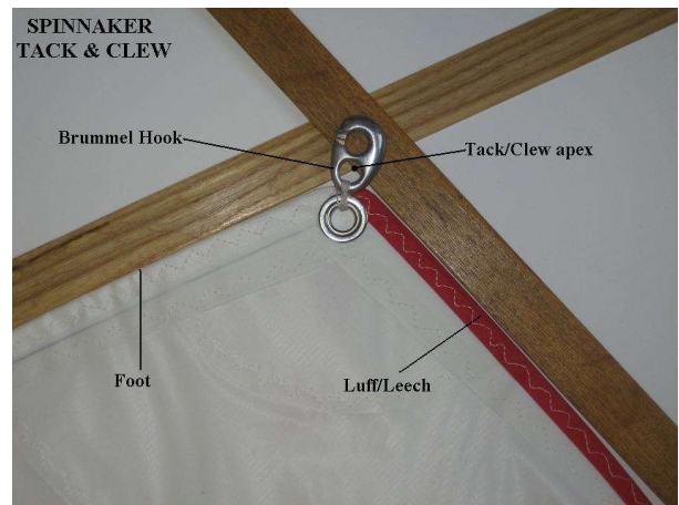
Photo 9 - Spinnaker Clew
