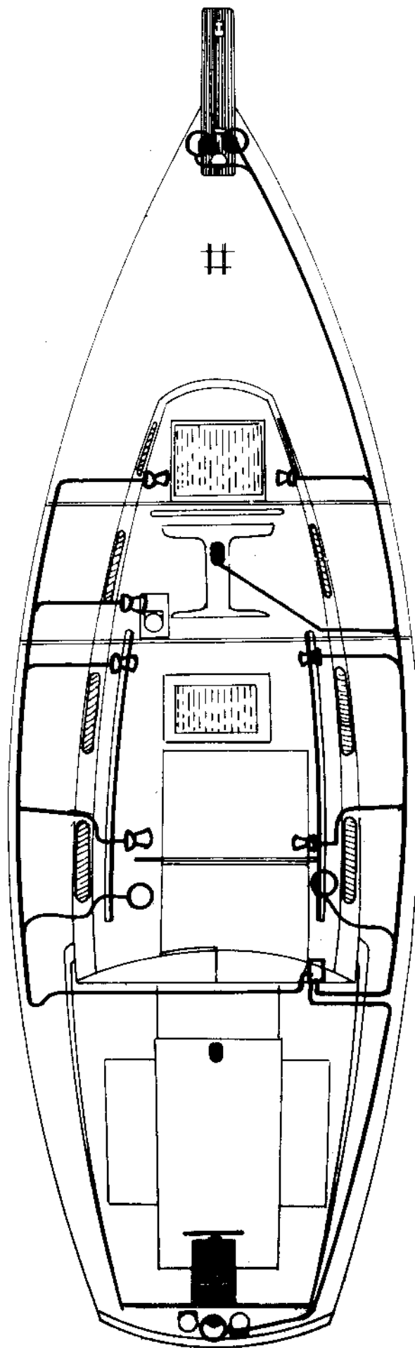
CAPE DORY 30-WIRING SYSTEM
