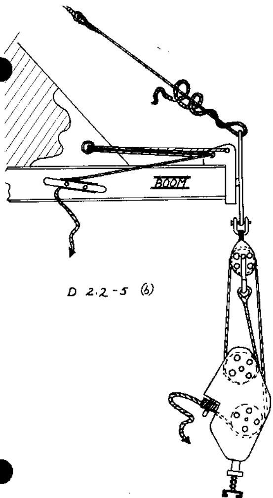
C.D. 25 MAINSHEET
