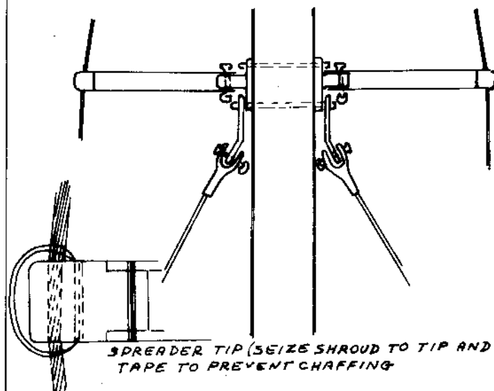
SPREADER ASSEMBLY
