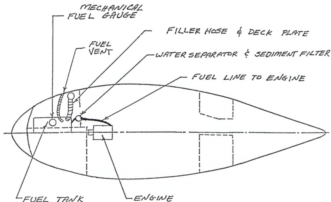
Figure 10 - Fuel Tank Installation
