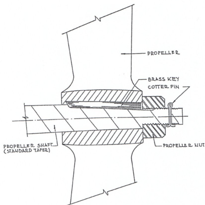
Figure 12 - Standard 2-Blade Propeller
