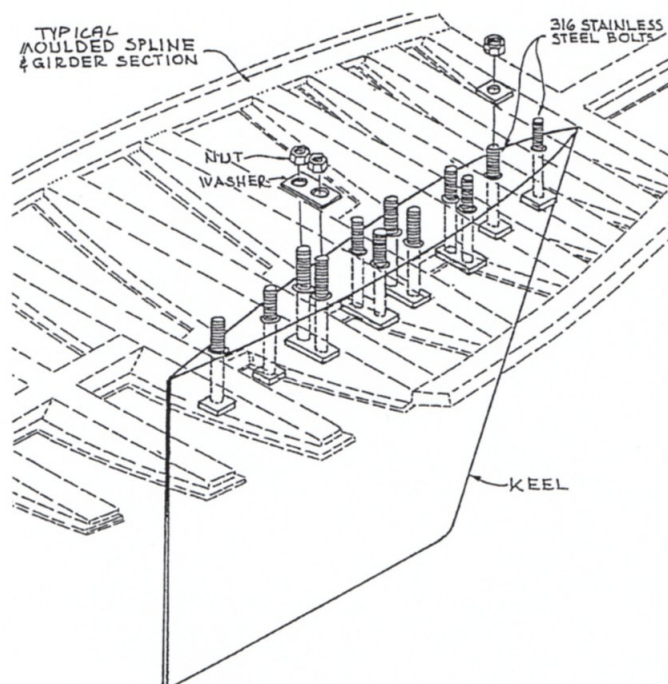
Figure 6 - Typical Keel Attachment
