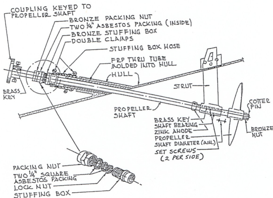
Figure 11 - Propeller Shaft & Stuffing Box
