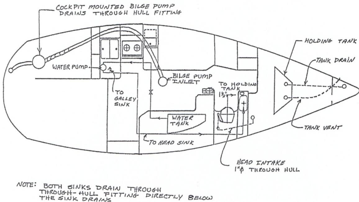
Figure 5 - General Plumbing Schematic
