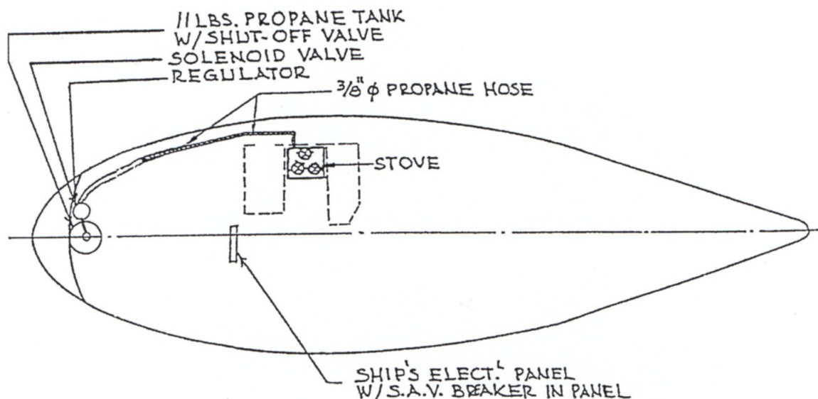
Figure 1 - Propane System with Solenoid Actuated Valve
