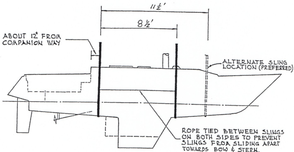
Figure 3 - Haulout Sling Location
