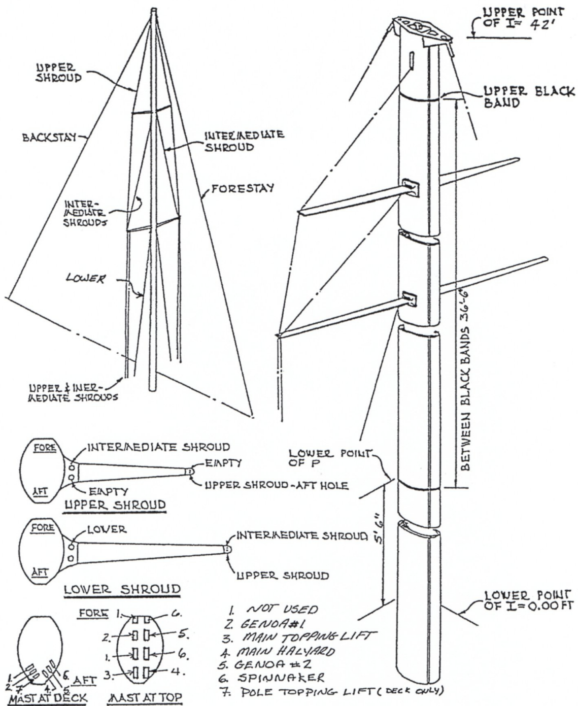
Figure 7 - Mast & Rigging Layout
