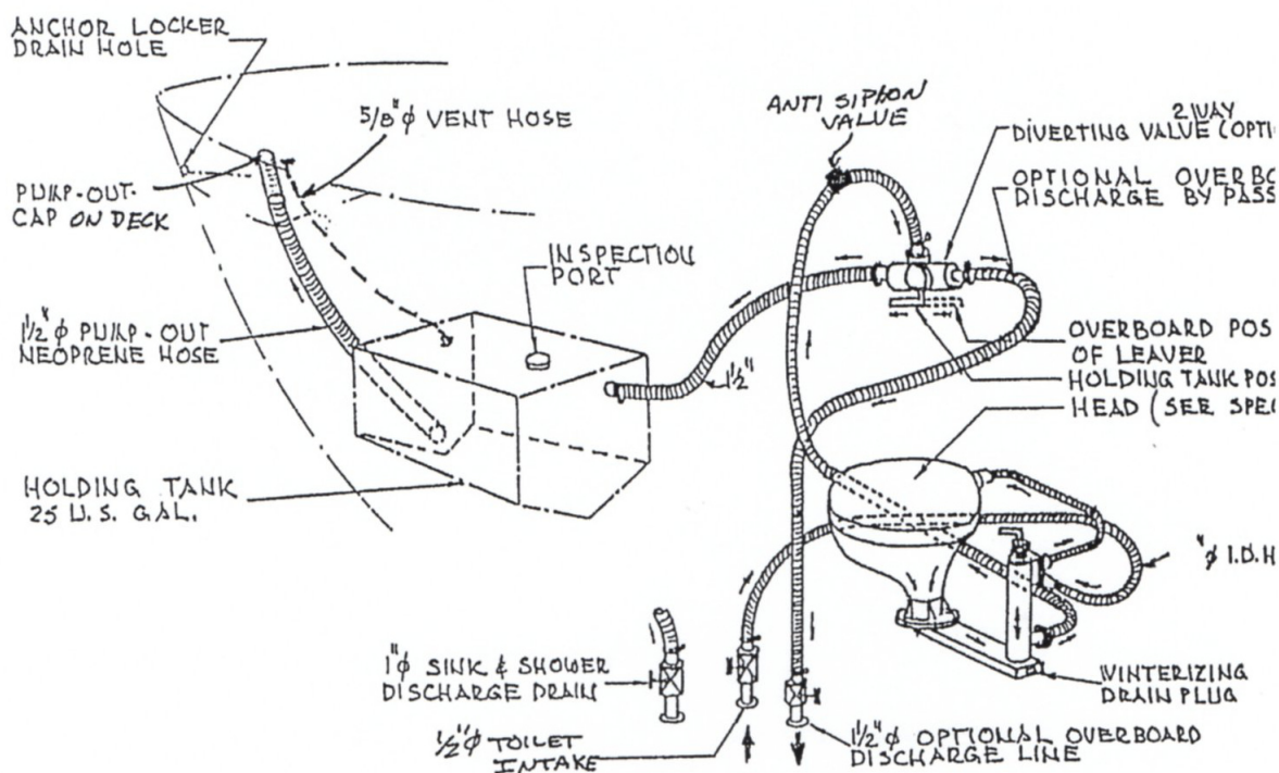
Figure 4 - Toilet Plumbing System
