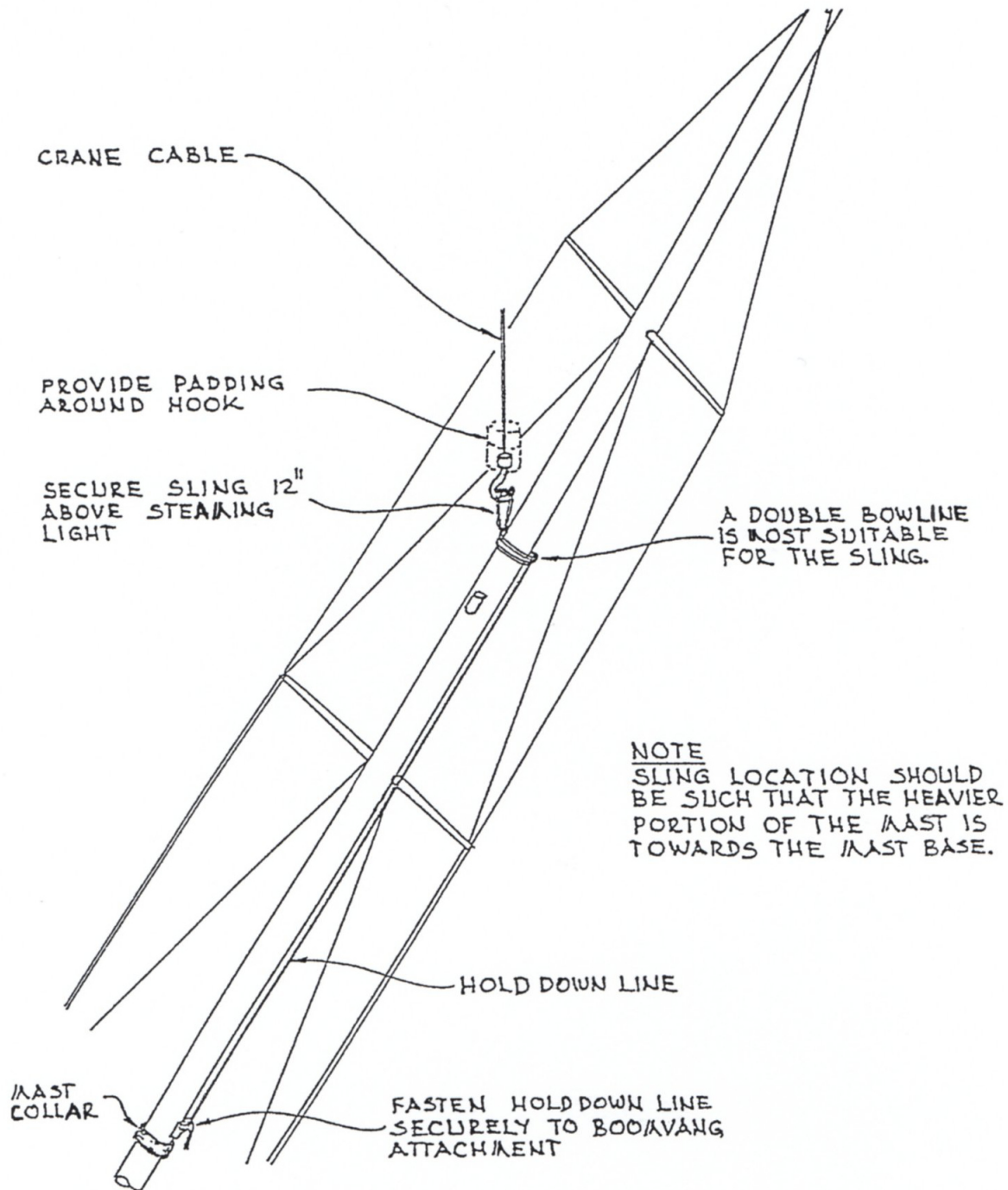
Figure 2 - Mast Sling Location
