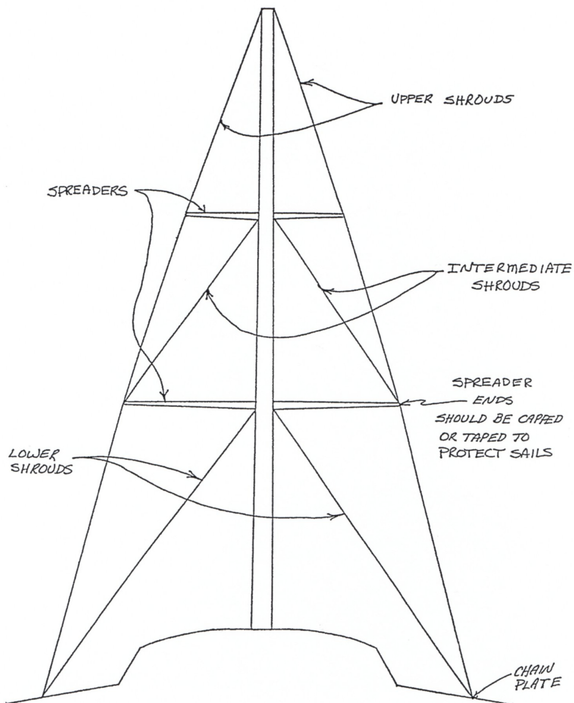
Figure 8 - Spreader Arrangement
