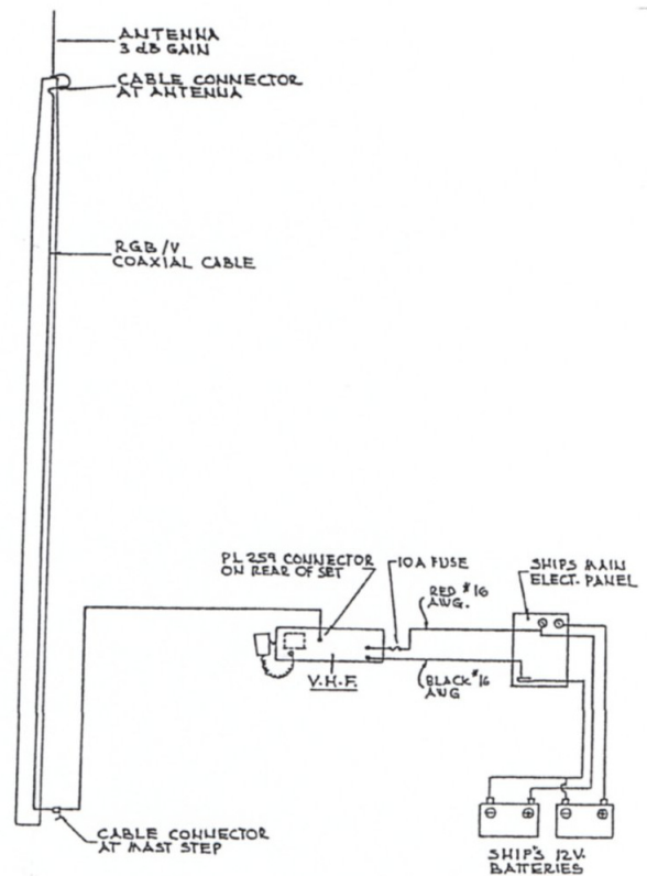
Figure 14 - VHF Radio Connections
