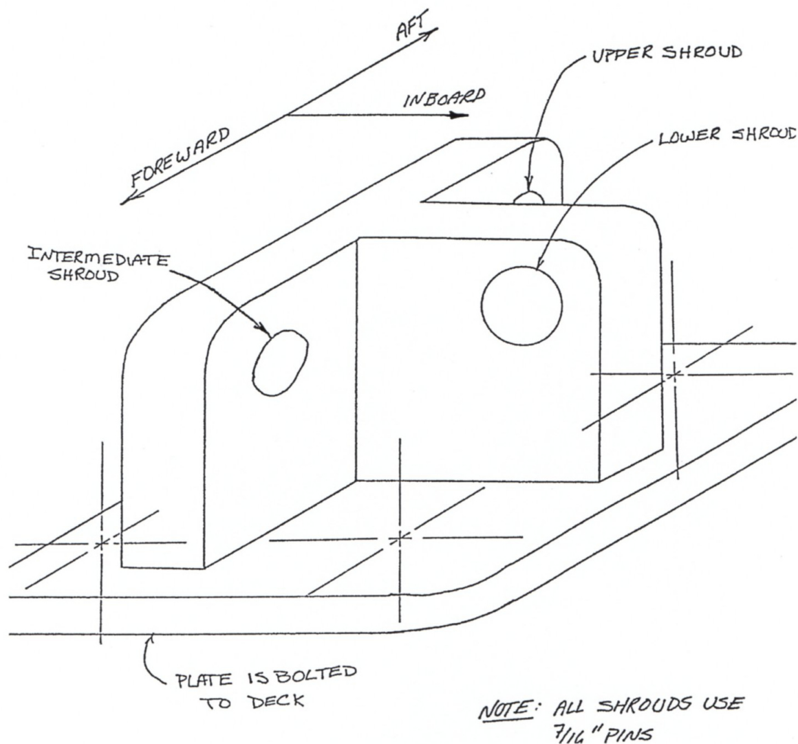
Figure 9 - Chainplate & Shroud Detail
