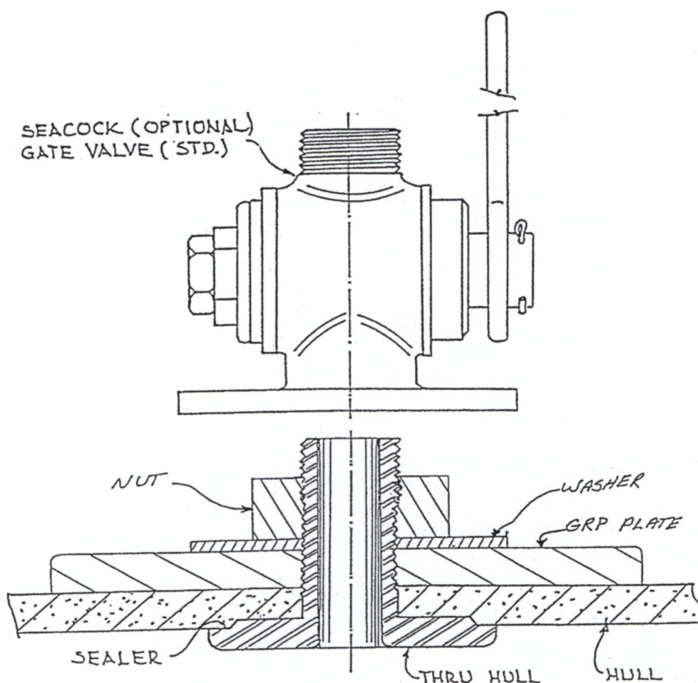
Figure 15 - Through Hull Fitting
