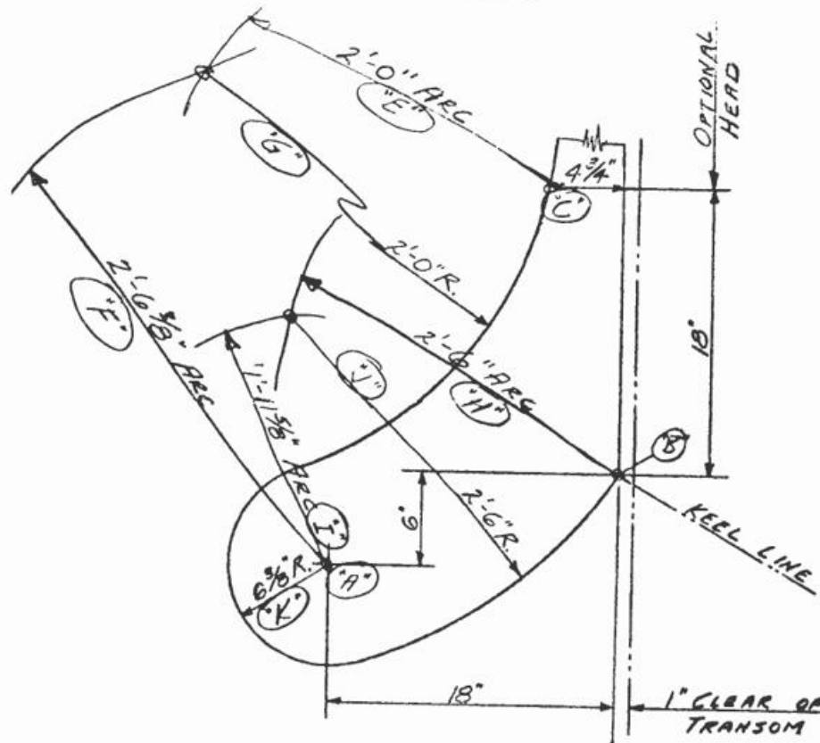
FIGURE 2. RUDDER SHAPE--CLASS X
