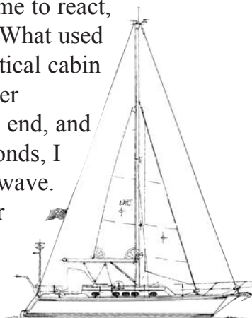
Heavy weather sail plan-Centered and high allows green water to pass under.
