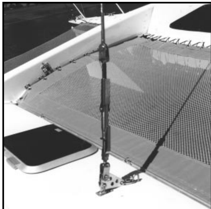
Link plate system on the F-28. Pulling the lower left clevis pin releases the shroud, but it remains secured to the float by the link to the u-bolt to the right, while allowing just enough slack for the float to fold (see page 24).
