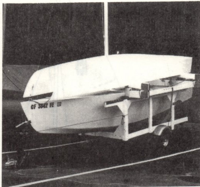
PICTURE SHOWING FLOATS IN FOLDED POSITION FOR STORING. MAST ALSO FOLDS FOR TRAILERING.
