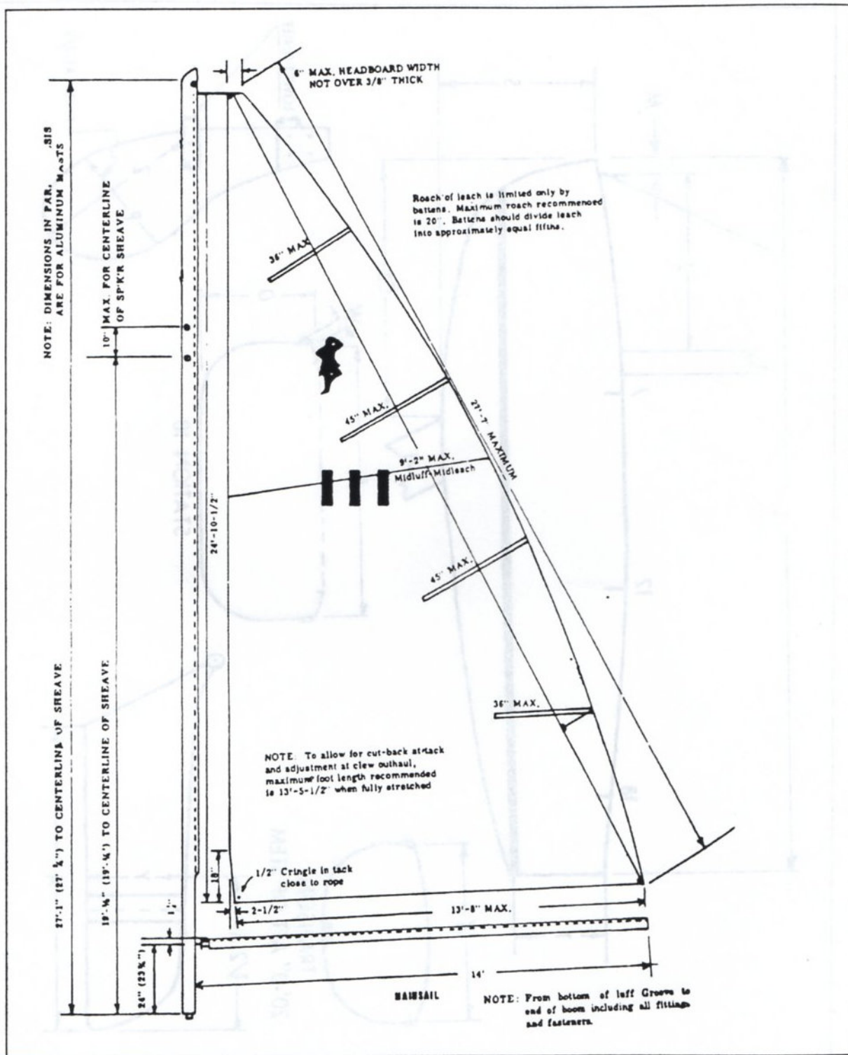
Figure 2 Mast, Boom and Mainsail Measurements
