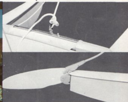
Controllable kick-up rudders
