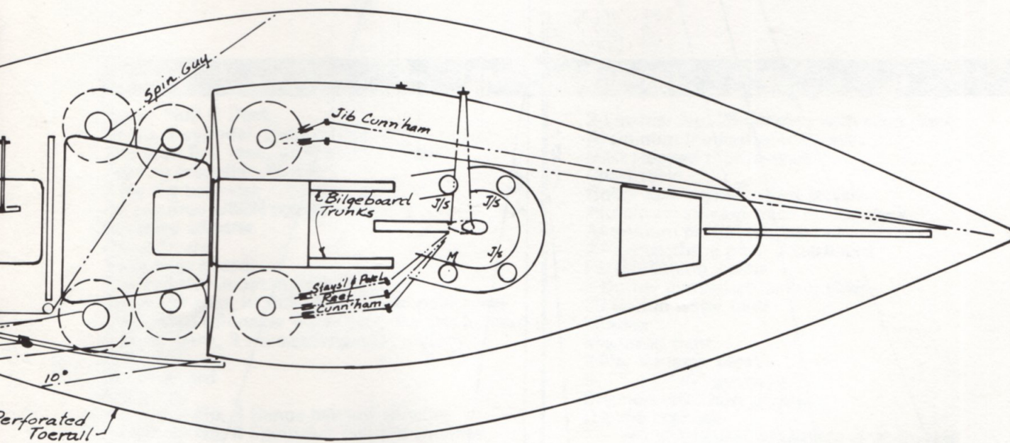
DECK & WINCH LAYOUT
