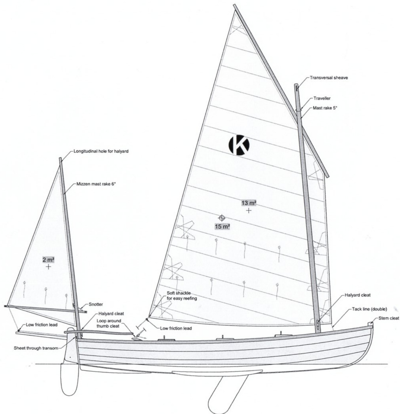
Kernic - Plan 41 Sail plan (lug yawl rig) Scale 1/30 28 December 2016 François Vivier Architecte Naval
