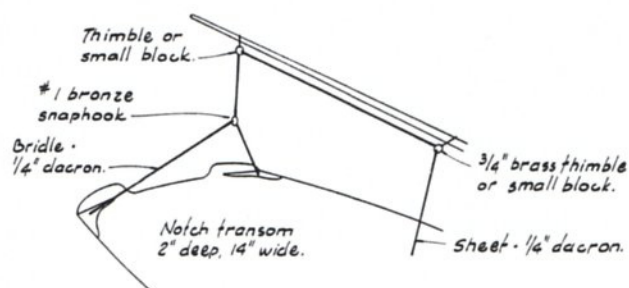
DETAIL of TRANSOM & SHEET
