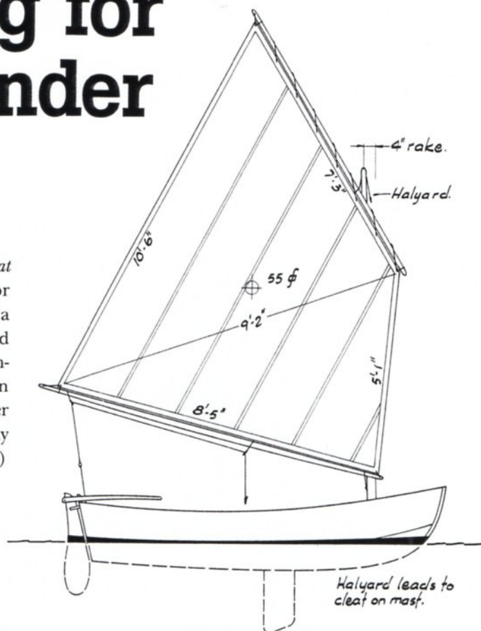
SAIL PLAN
