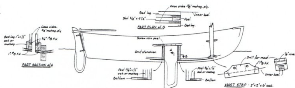
CONSTRUCTION PROFILE
