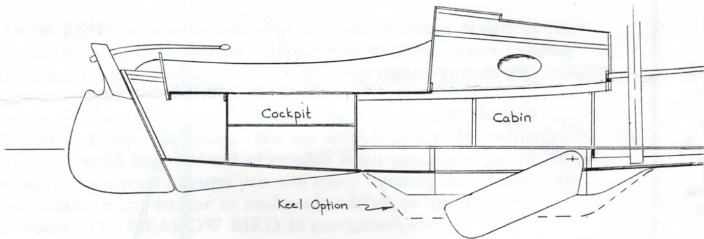
INBOARD PROFILE
