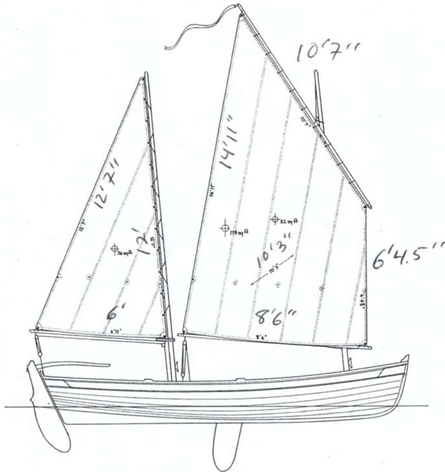
KETCH RIG
