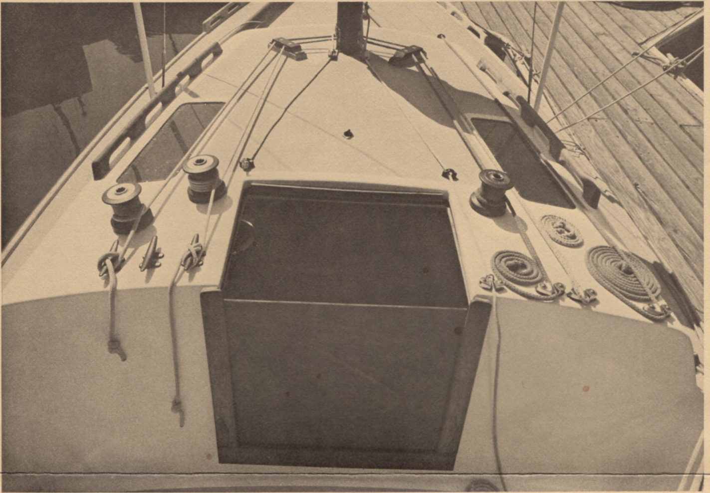
CABIN TOP ON "CALIFORNIA ZYPHER" SHOWING CABIN TOP, WINDOWS AND ALL HALYARDS LEADING AFT. TO COCKPIT.
