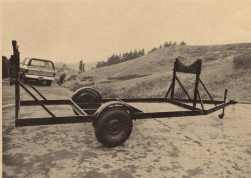
CUSTOM TRAILER WITH SURGE BRAKES
