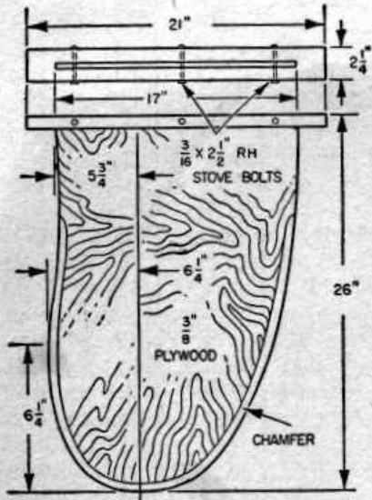
CENTER BOARD 1" DIA. HOLE
