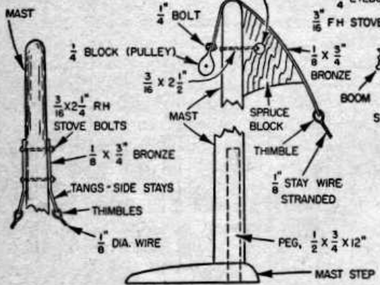
MAST HEAD DETAILS
