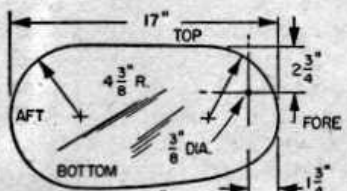
RUDDER BLADE - 1/16 SHEET METAL (OR HEAVIER ALUMINUM) 2" #10 FH SCREWS C/SUNK
