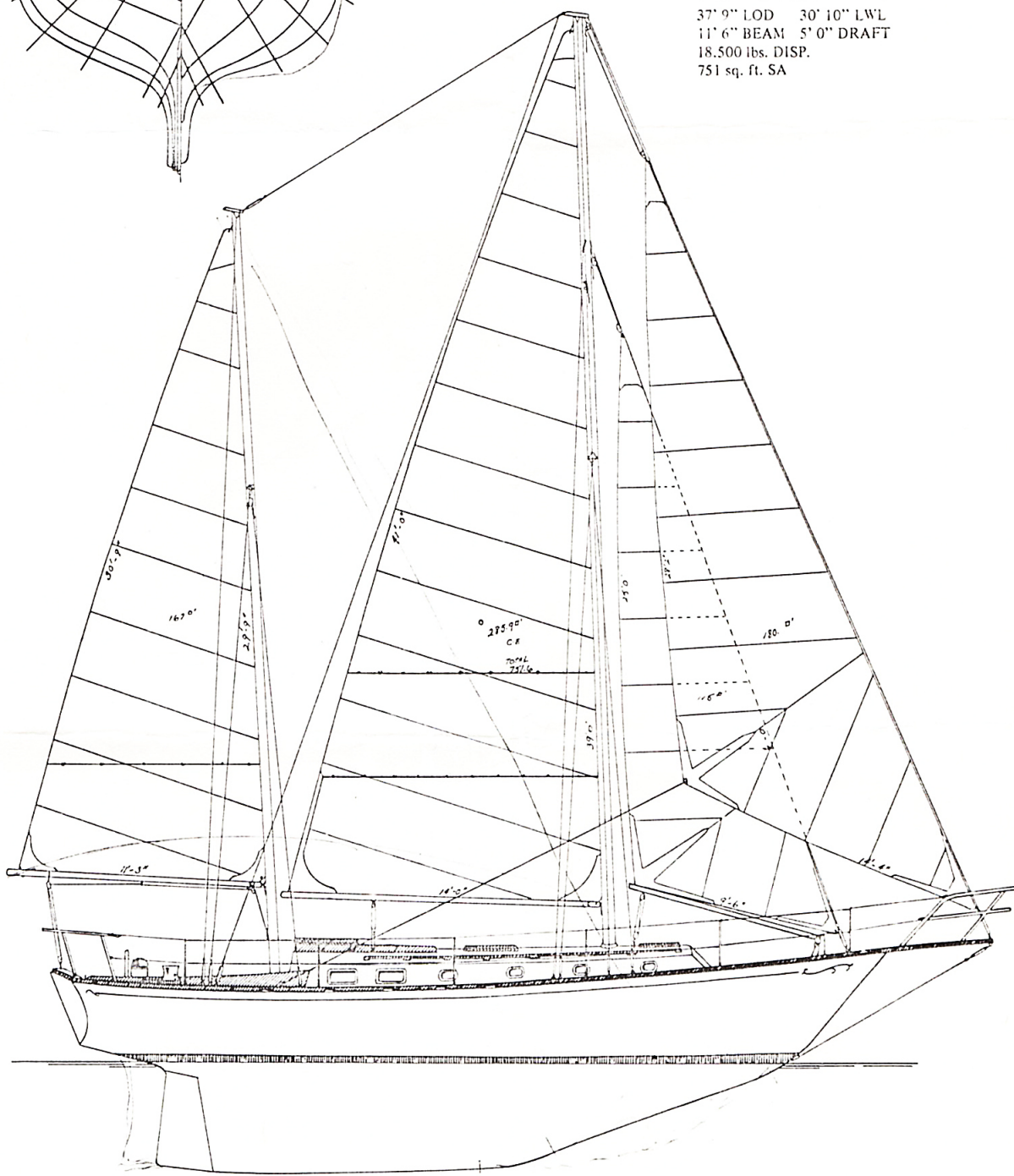
SHANNON 38 KETCH
