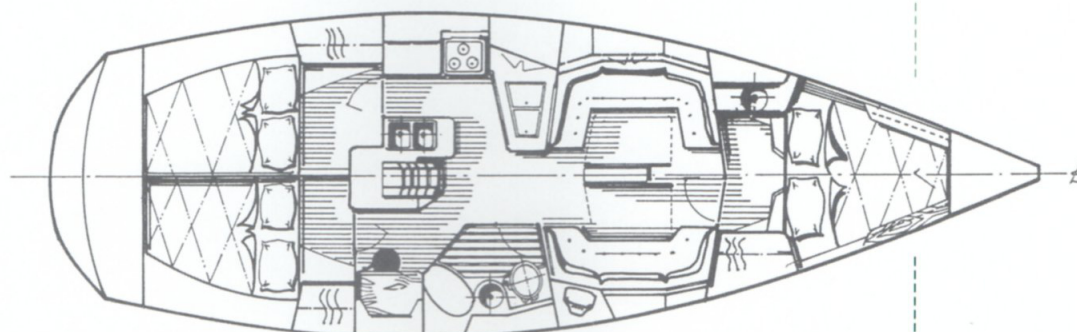
Optional Tri-Cabin Arrangement
