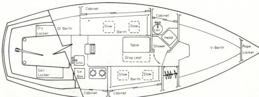
Watkins 27
