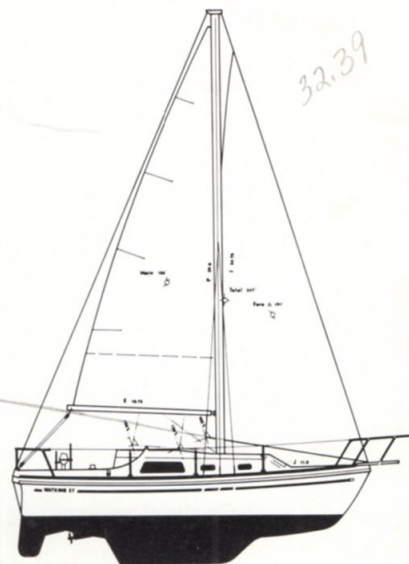
Watkins 27
