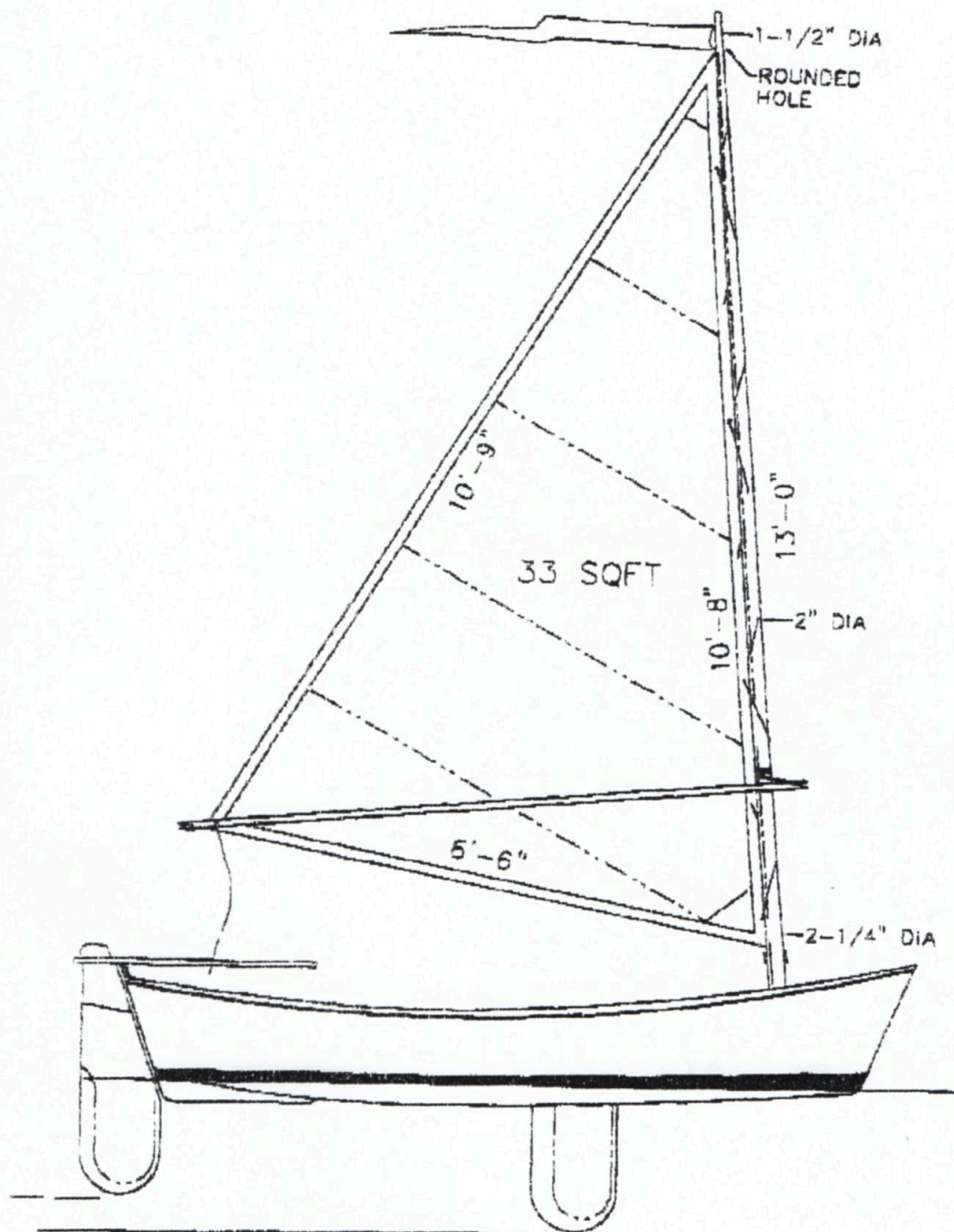
SAIL PLAN
