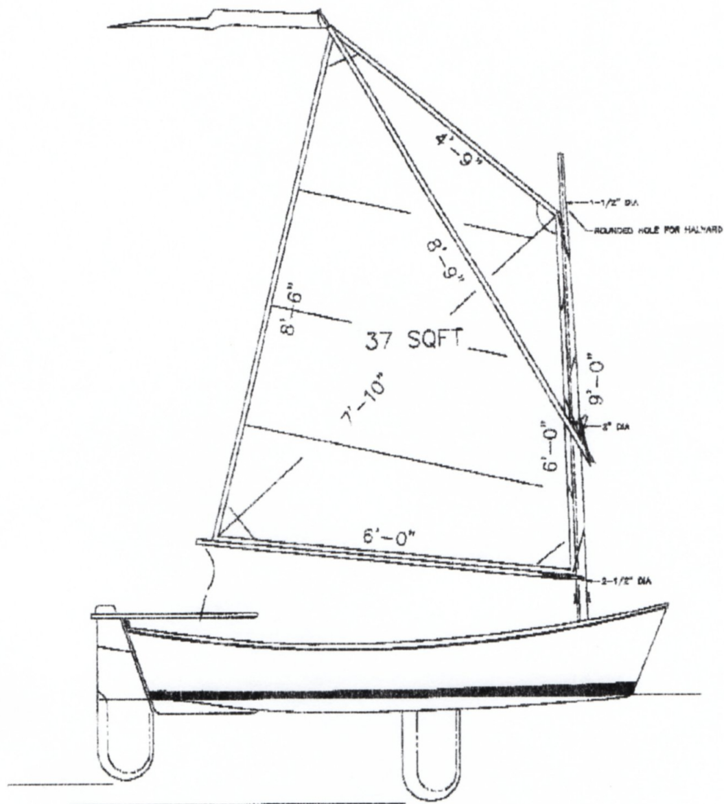
SAIL PLAN
