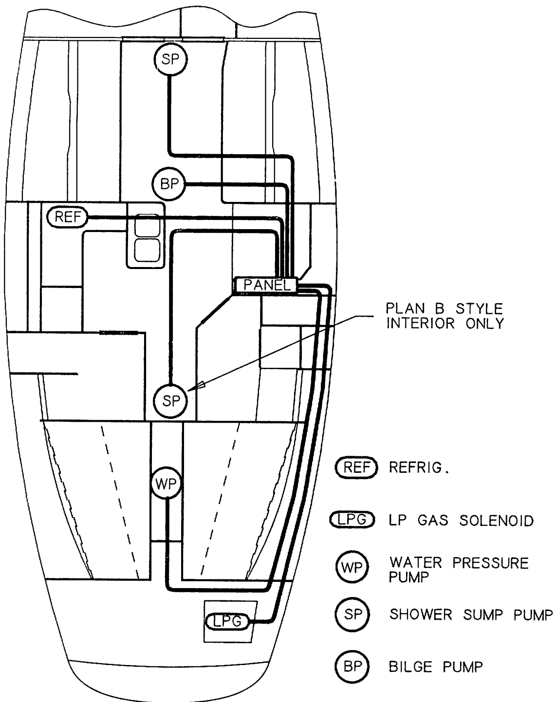
J/44 12V DC EQUIPMENT- FIG. 13
