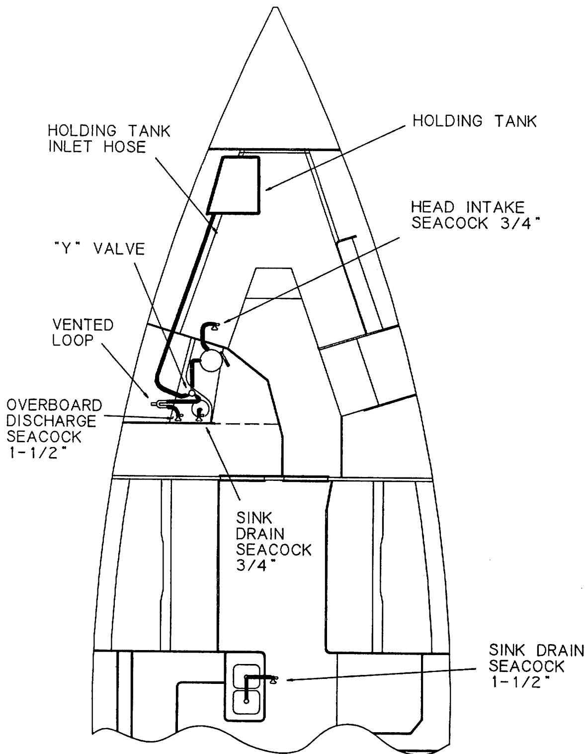
J/44 HEAD LAYOUT- FIG. 11a
