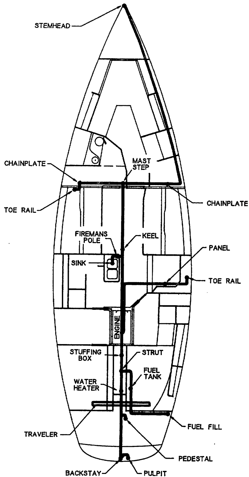
J/44 BONDING SYSTEM- FIG. 16
